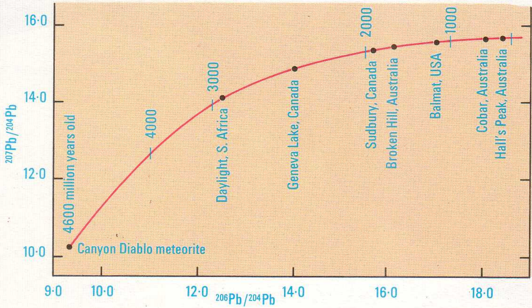
43 Lead ratios and the age of the Earth
